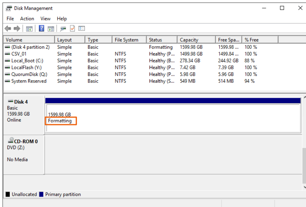
Figure 16 Avoid long format wait times by temporarily disabling trim/unmap
