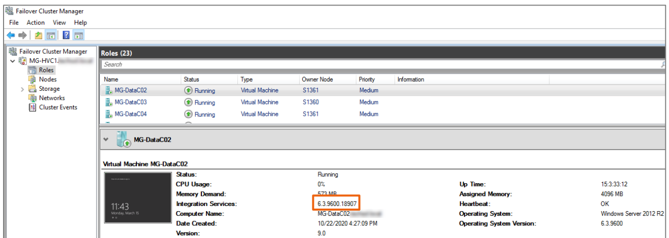
Figure 6 Verify integration services version with Failover Cluster Manager
