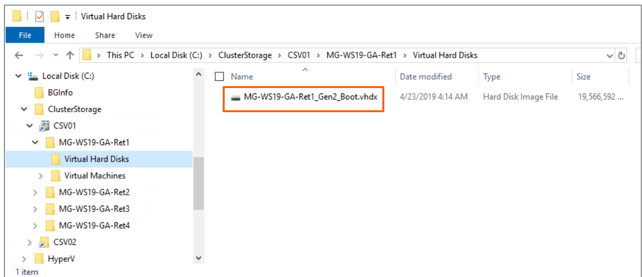
Figure 9 A boot virtual hard disk file (vhdx) for a Windows Server 2019 guest VM on a cluster shared volume
