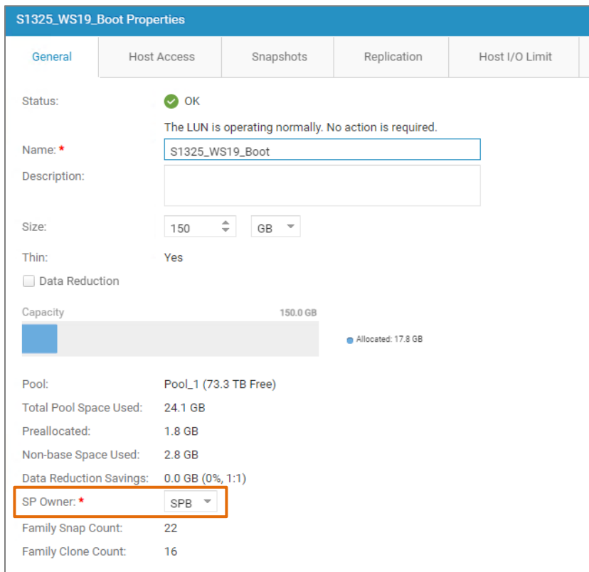
Figure 20 View or change the storage processor owner for a LUN
