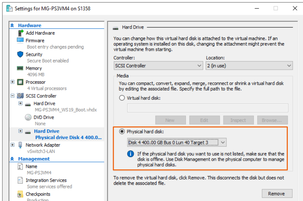
Figure 15 Add a Unity volume to a guest VM as a pass-through disk
