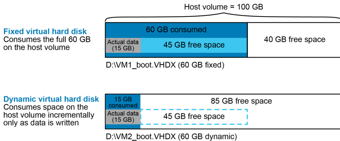
Figure 12 Fixed and dynamic virtual hard disk comparison
