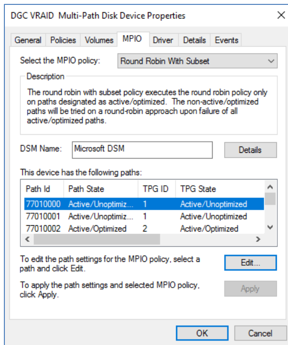
Figure 14 Verify MPIO settings (Microsoft DSM shown)
