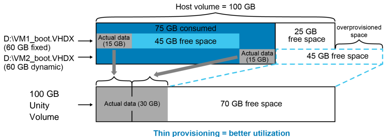
Figure 13 Thin provisioning with Unity
